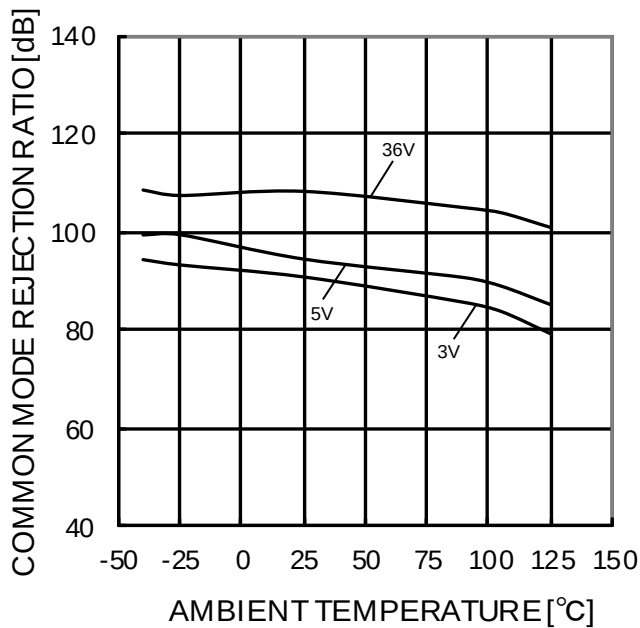
Figure 96. 同相信号除去比－温度特性
