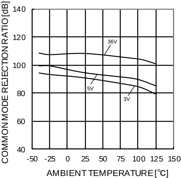
Figure 72. 同相信号除去比－温度特性
