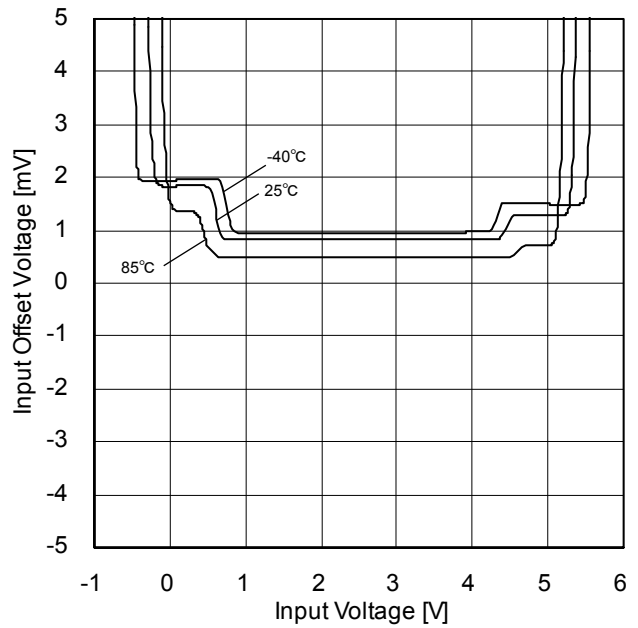
Figure 14. 同相入力電圧 (V+=5V)
