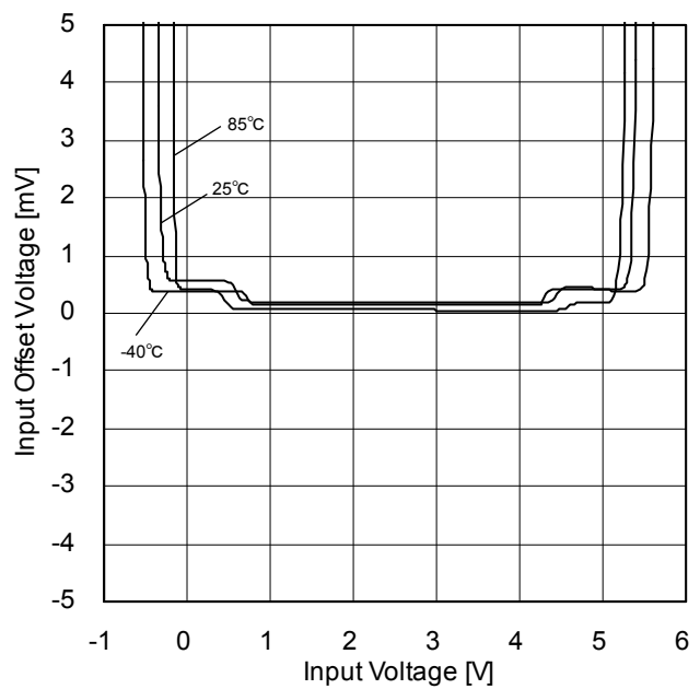
Figure 67. 同相入力電圧 (V+=5V)
