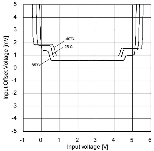
Figure 40. 同相入力電圧 (V+=5V)
