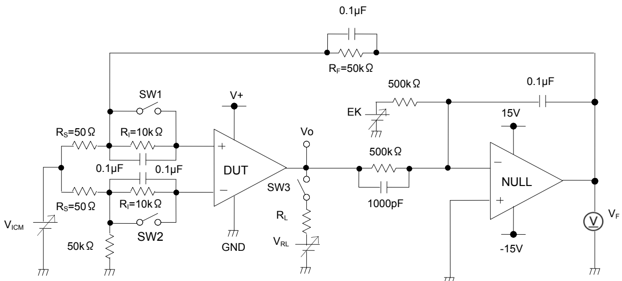
Figure 81. 測定回路 1
