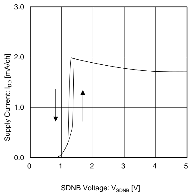
Figure 29. 回路電流 vs SDNB 電圧 ( V_S = 5\text{ V} , V_{ICM} = 2.5\text{ V} , G = 0\text{ dB} )
