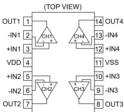
BD7284FV-LB (SSOP-B14) BD7284F-LB (SOP14)
