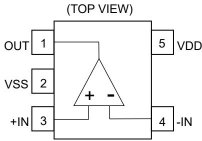
BD7281G-LB (SSOP5)
