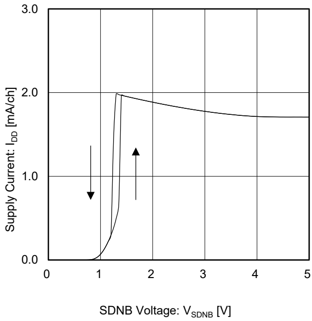
Figure 29. 回路電流 vs SDNB 電圧 ( V_S = 5\text{ V} , V_{ICM} = 2.5\text{ V} , G = 0\text{ dB} )
