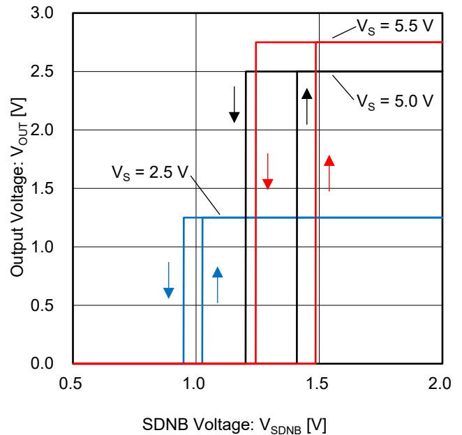
Figure 28. 出力電圧 vs SDNB 電圧 ( V_{ICM} = V_S/2 , G = 0\text{ dB} )
