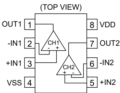
BD7282FVM-LB (MSOP8) BD7282FJ-LB (SOP-J8)
