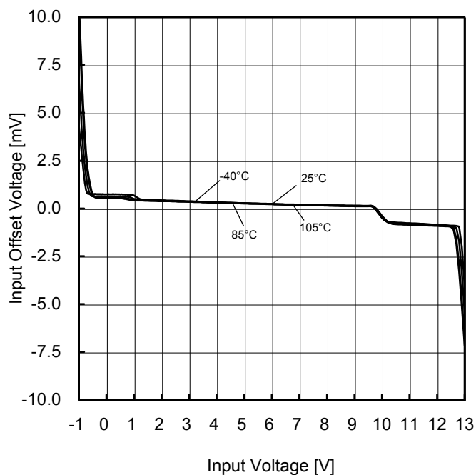
Figure 39. 同相入力電圧範囲 ( V_{DD}=12V )
