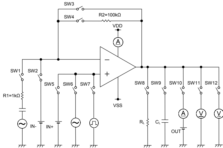
Figure 49. 測定回路 2
