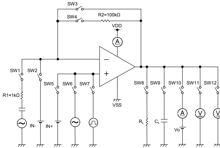
Figure 72. 測定回路 2
