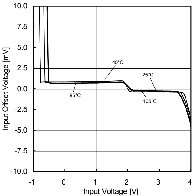
Figure 62. 同相入力電圧範囲 ( V_{DD} = 3[V] )
