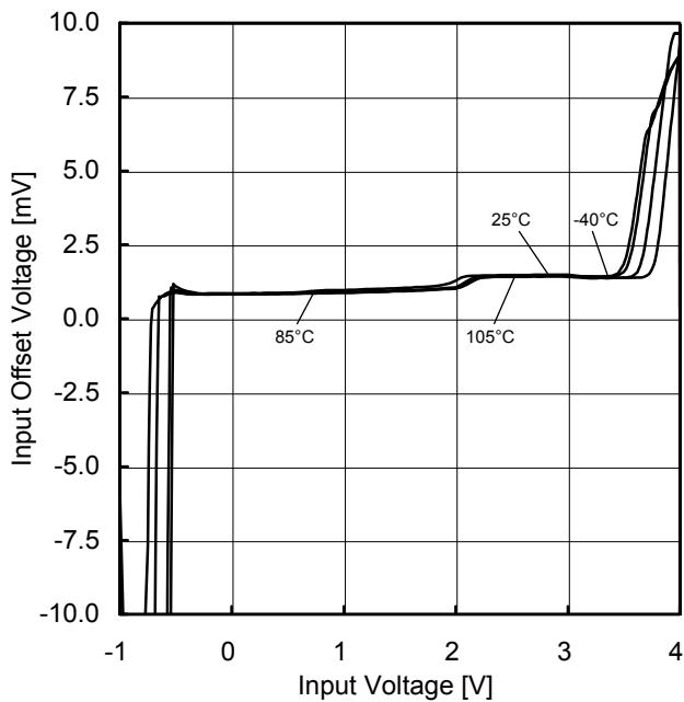
Figure 39. 同相入力電圧範囲 ( V_{DD}=3V )
