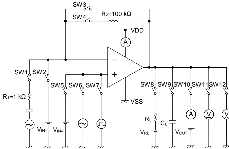
Figure 31. 測定回路 2
