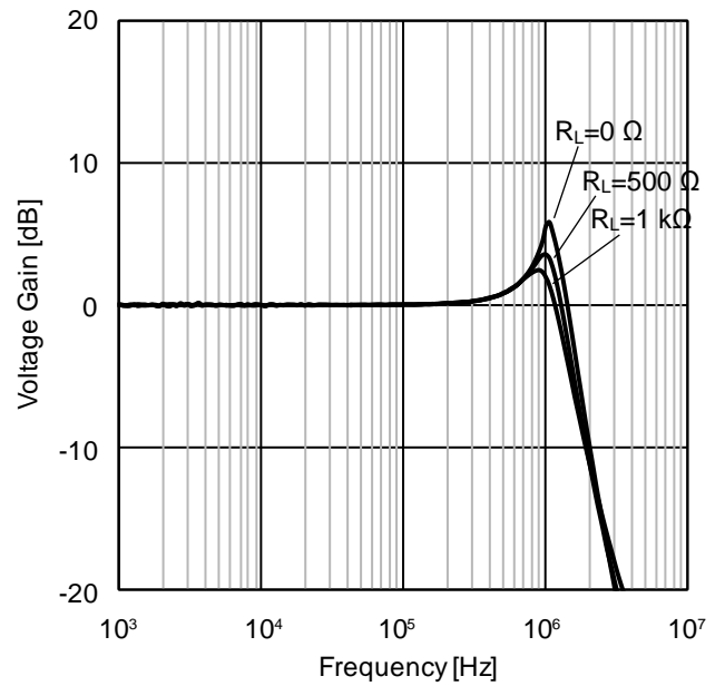
Figure 41. 電圧利得 vs 周波数特性 ( V_{DD}=3.0\text{ V}, G_V=0\text{ dB}, C_L=100\text{ pF}, \text{Circuit: Figure 39} )
