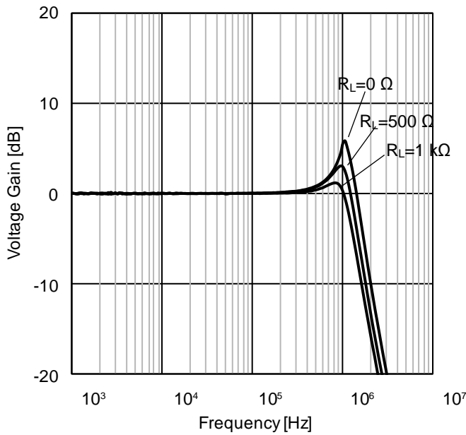
Figure 40. 電圧利得 vs 周波数特性 ( V_{DD}=3.0\text{ V}, G_V=0\text{ dB}, C_L=100\text{ pF}, \text{Circuit: Figure 38} )
