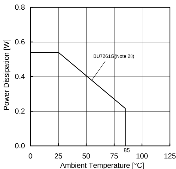
(c)BU7261G
