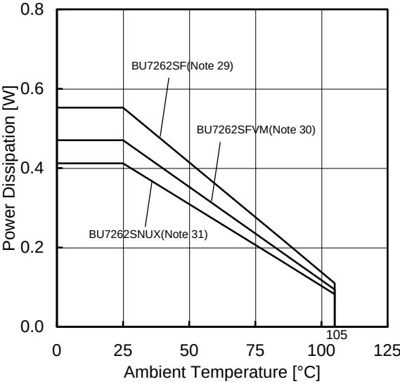
(f)BU7262SF/SFVM/SNXX
