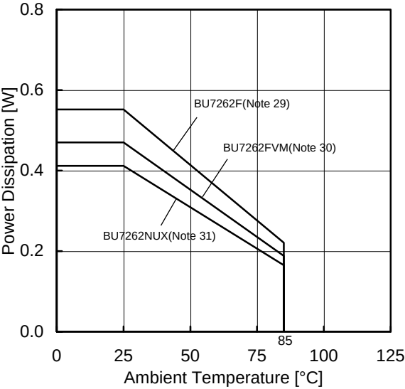
(e)BU7262F/FVM/NUX
