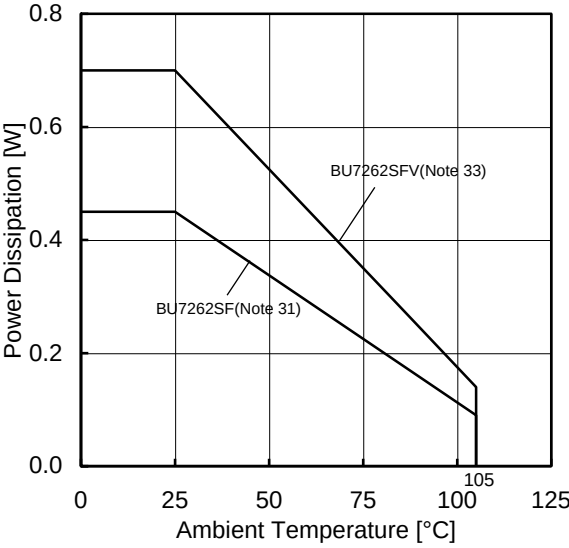
(h)BU7264SF/SFV
