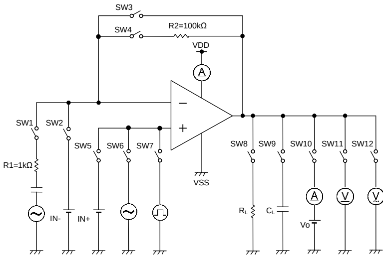
Figure 72. 測定回路 2
