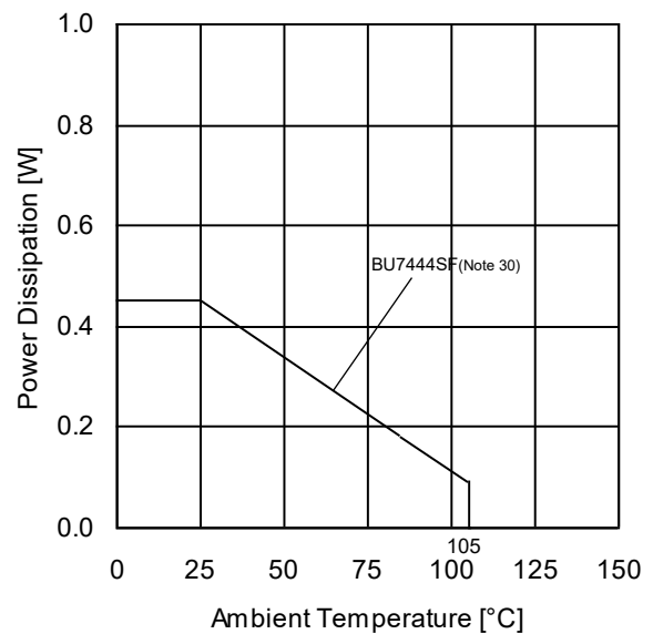
(h) BU7444SF
