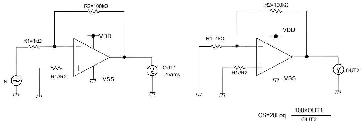
Figure 74. 測定回路 3
