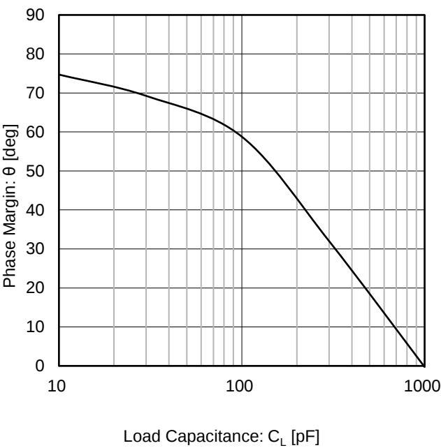
Figure 29. 位相余裕 vs 負荷容量 ( V_S = 2.7\text{ V} , R_F = 10\text{ k}\Omega , G = 40\text{ dB} )
