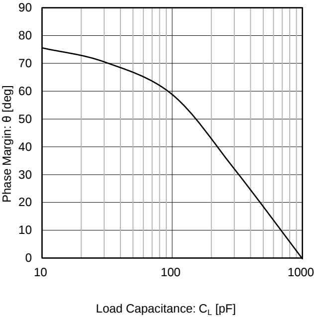
Figure 30. 位相余裕 vs 負荷容量 ( V_S = 5\text{ V} , R_F = 10\text{ k}\Omega , G = 40\text{ dB} )
