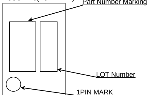
TSSOP-B8(TOP VIEW)
