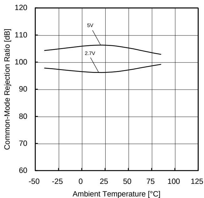
Figure 64. 同相信号除去比－温度特性
