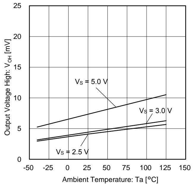
Figure 4. 出力電圧 High vs 温度 ( R_L = 10\text{ k}\Omega , V_{OH} = V_{DD} - V_{OUT} )
