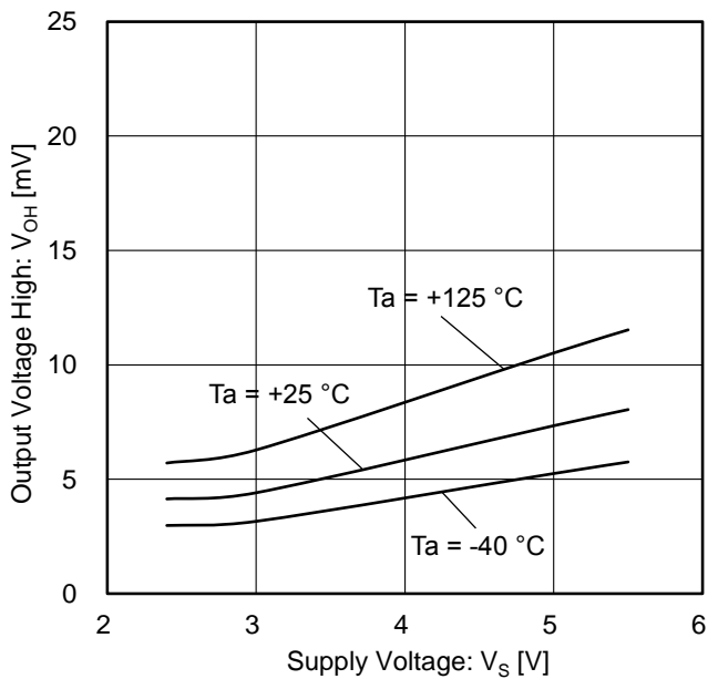
Figure 3. 出力電圧 High vs 電源電圧 ( R_L = 10\text{ k}\Omega , V_{OH} = V_{DD} - V_{OUT} )
