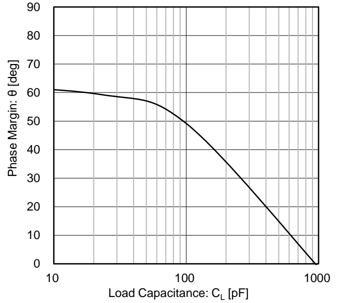
Figure 18. 位相余裕 vs 負荷容量 ( V_S = 5\text{ V} , R_F = 10\text{ k}\Omega , G = 40\text{ dB} )
