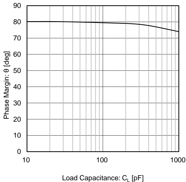
Figure 23. 位相余裕 vs 負荷容量 ( V_S = 3\text{ V} , R_F = 5\text{ M}\Omega , G = 20\text{ dB} )
