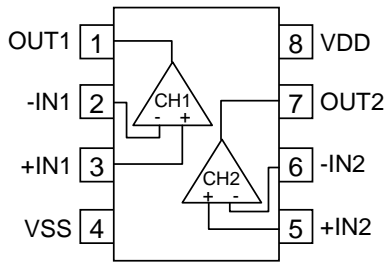
TLR2372YFJ-C (SOP-J8)
