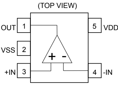
TLR728G-LB (SSOP5)
