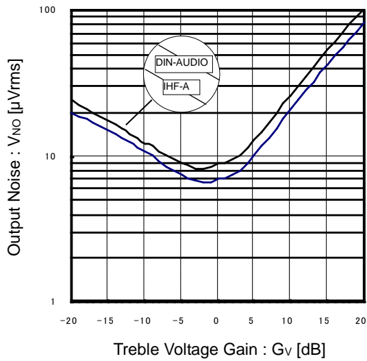
Figure 11. Output Noise vs Treble Gain
