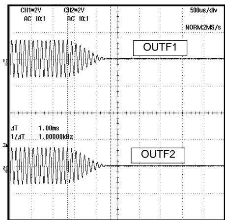
Figure 15. Advanced Switch 2
