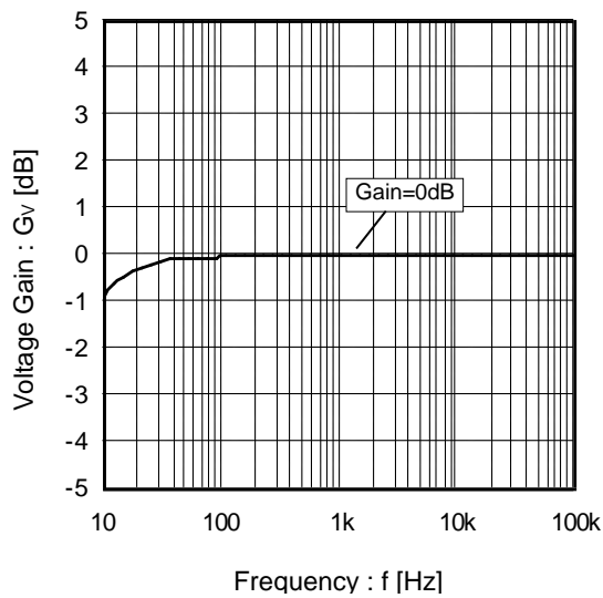
Figure 3. Voltage Gain vs Frequency
