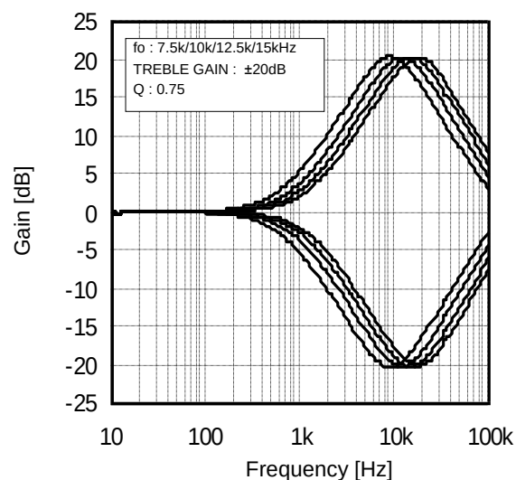
Figure 8 Treble fo vs Frequency
