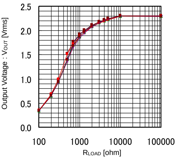
Figure 14. Output Voltage vs R_LOAD
