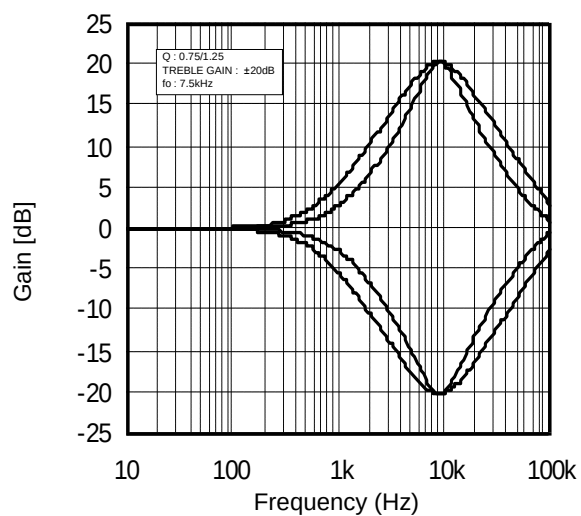
Figure 9. Treble Q vs Frequency
