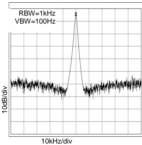
Figure 15. 22.6MHz Spectrum V DD =3.3V, at C L =15pF
