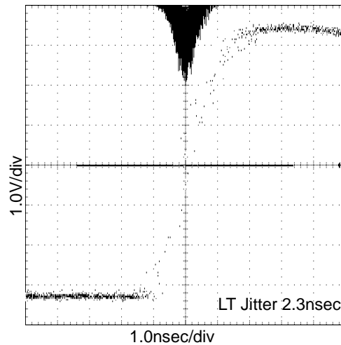
Figure 16. 24.6MHz LT Jitter V DD =3.3V, at C L =15pF
