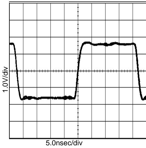
Figure 13. 22.6MHz Output Waveform V DD =3.3V, at C L =15pF
