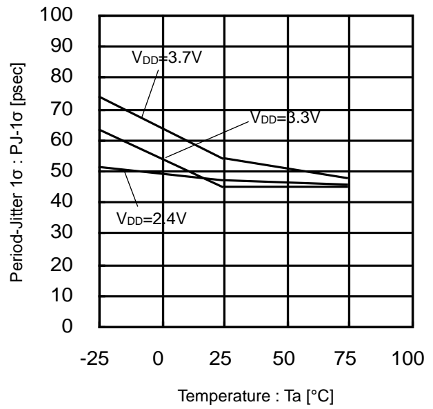
Figure 31. Period-Jitter 1σ vs Temperature (22.6MHz)
