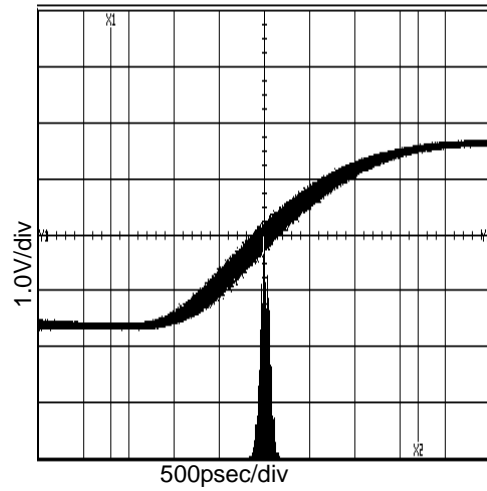
Figure 14. 22.6MHz Period-Jitter V DD =3.3V, at C L =15pF
