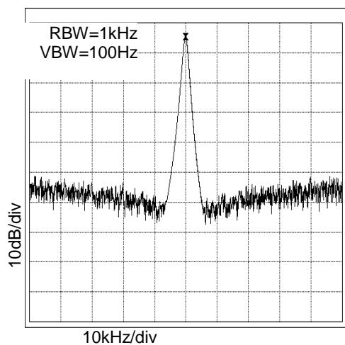
Figure 9. 33.9MHz Spectrum V_{DD}=3.3V , at C_L=15pF
