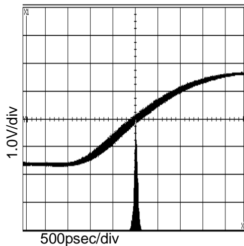
Figure 2. 54MHz Period-Jitter ( V_{DD}=3.3V , at C_L=15pF )
