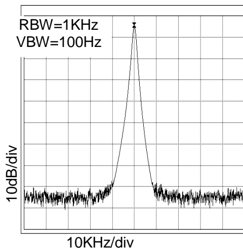
Figure 6. 27MHz Spectrum ( V_{DD}=3.3V , at C_L=15pF )
