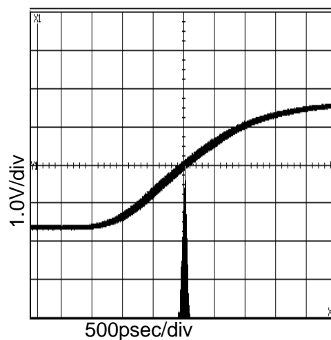
Figure 8. 33.9MHz Period-Jitter ( V_{DD}=3.3V , at C_L=15pF )
