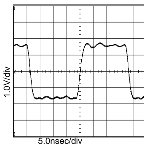
Figure 4. 27MHz Output Waveform ( V_{DD}=3.3V , at C_L=15pF )
