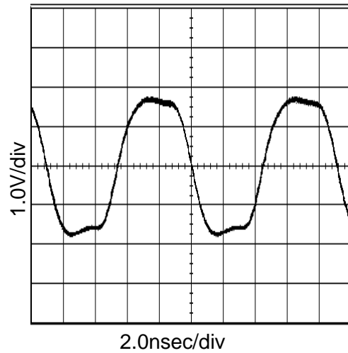
Figure 4. 110MHz Output Wave (At V_{DD}=3.3V and C_L=15pF )
