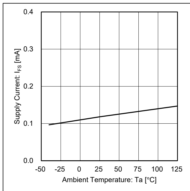
Figure 5. Supply Current vs Ambient Temperature (VFS Current Consumption)
