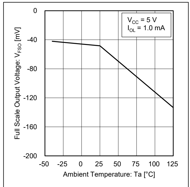
Figure 19. Full Scale Output Voltage vs Ambient Temperature
