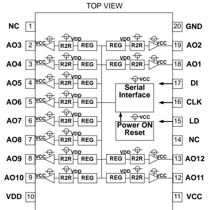
Figure 2. BH2221FV
