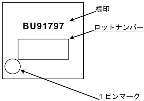
VQFN48FV7070 (TOP VIEW)
