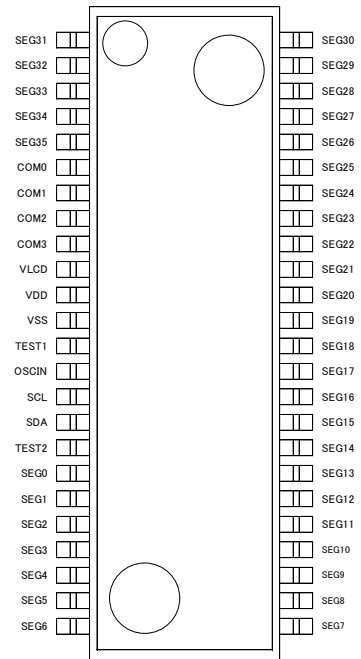
Figure 5. 端子配置図 (TOP VIEW)
