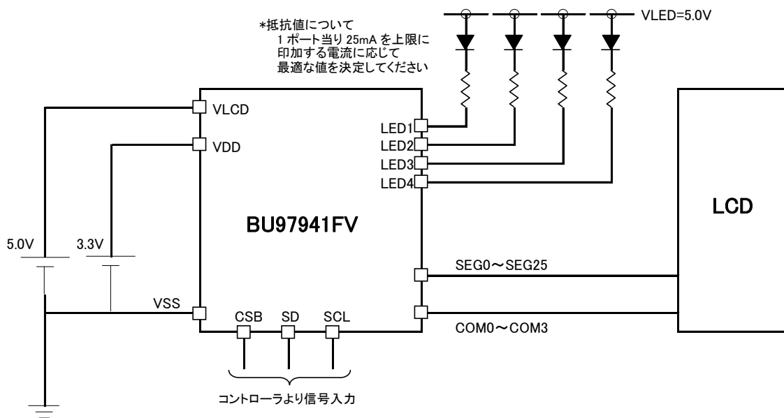
Figure 6. 推奨回路例
