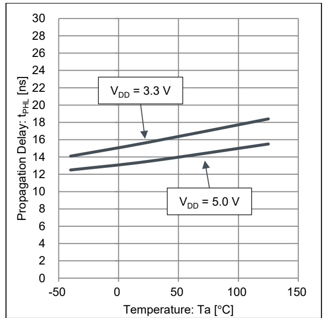
Figure 6. Propagation Delay (High to Low) vs Temperature
