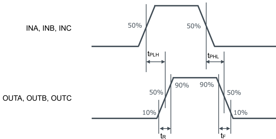
Figure 7. Input / Output Timing Chart
