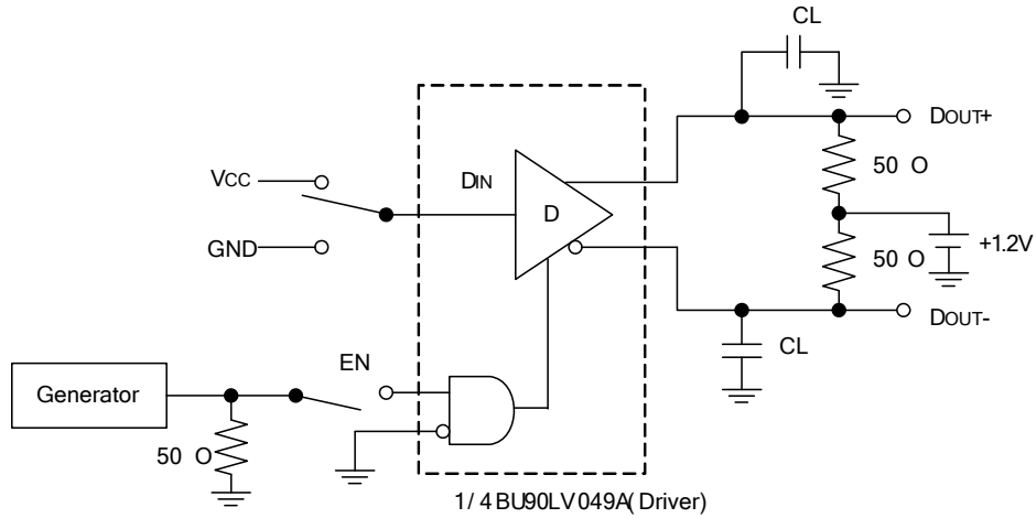
图-7 Driver 3-STATE Delay Test Circuit
