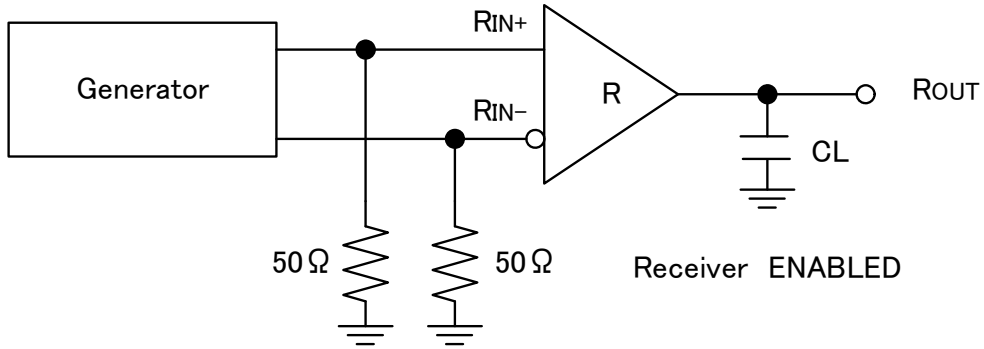
图-9 Receiver Propagation Delay and Transition Time Test Circuit
