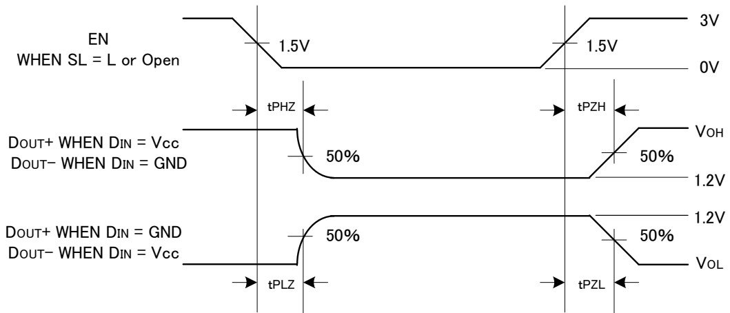
图-8 Driver 3-STATE Delay Waveform
