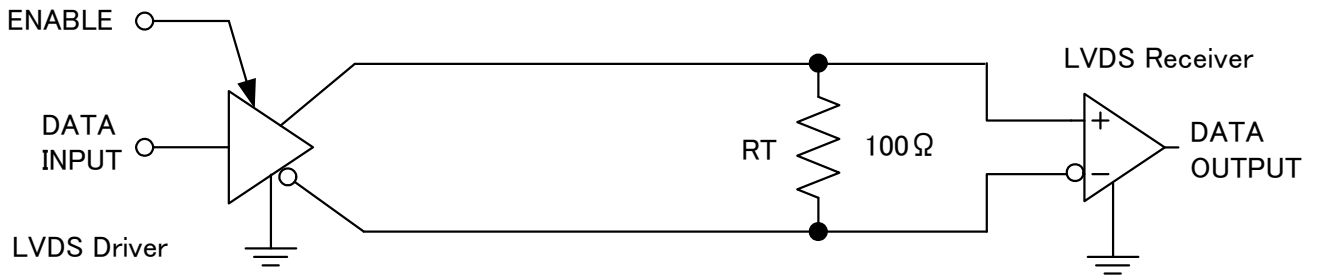
图-13 Point-to-Point Application
