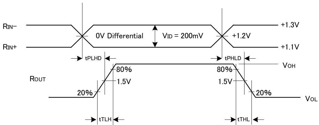
图-10 Receiver Propagation Delay and Transition Time Waveforms
