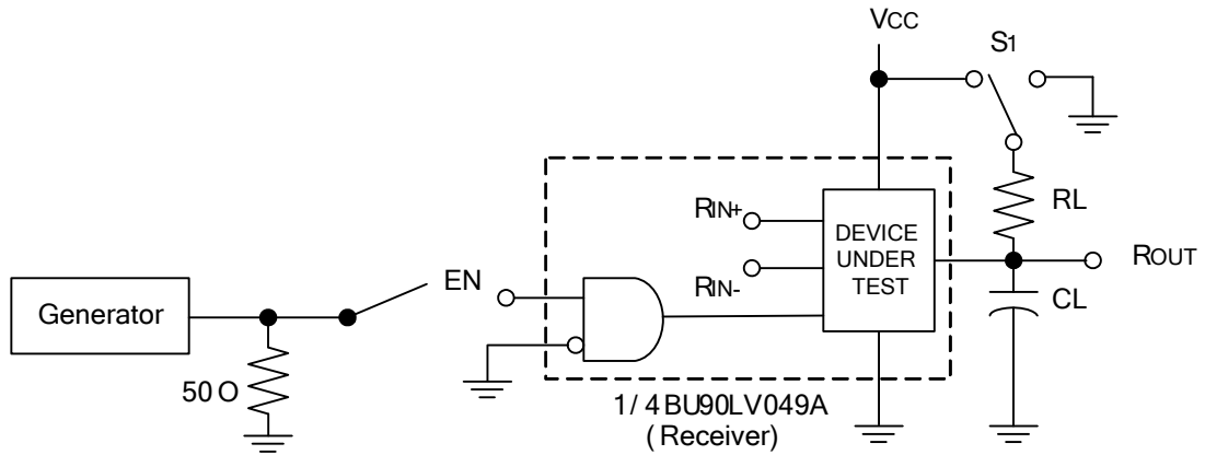
图-11 Receiver 3-STATE Delay Test Circuit
