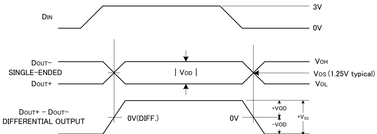
图-14 Driver Output Levels
