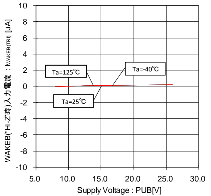
Figure 108. WAKB("Hi-Z")時入力電流-電圧特性
