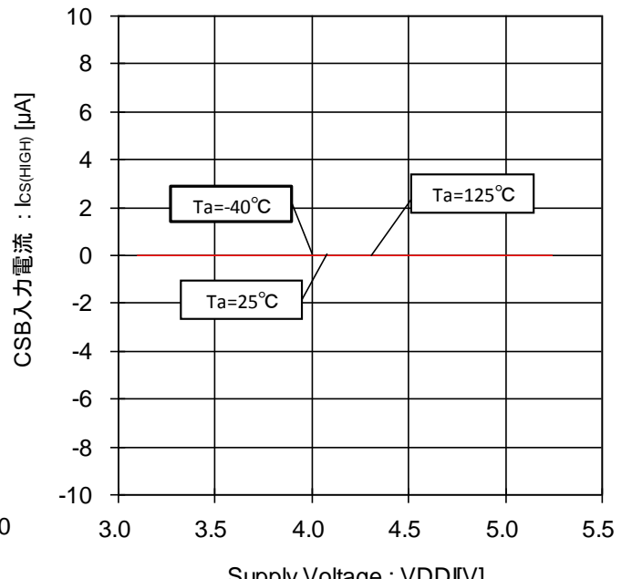
Figure 82. CSB 入力電流-電圧特性 (CSB=VDDI)
