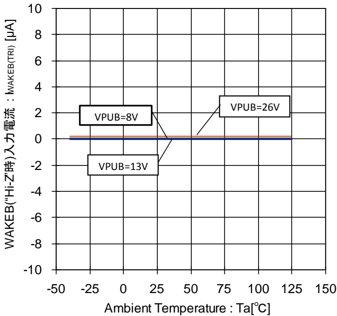
Figure 107. WAKB("Hi-Z")時入力電流-温度特性
