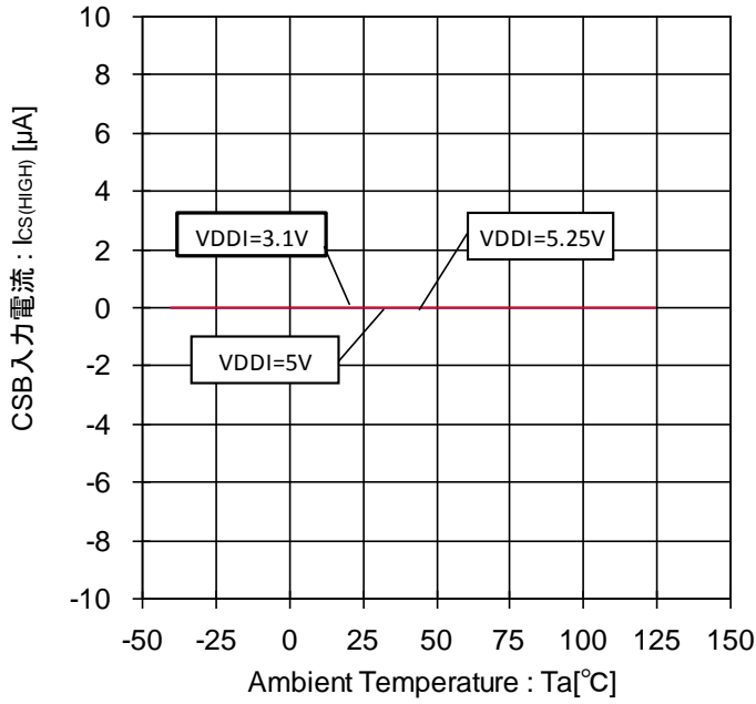
Figure 81. CSB 入力電流-温度特性 (CSB=VDDI)
