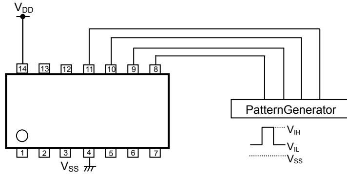
Figure 2. H/L 入力電圧測定回路
