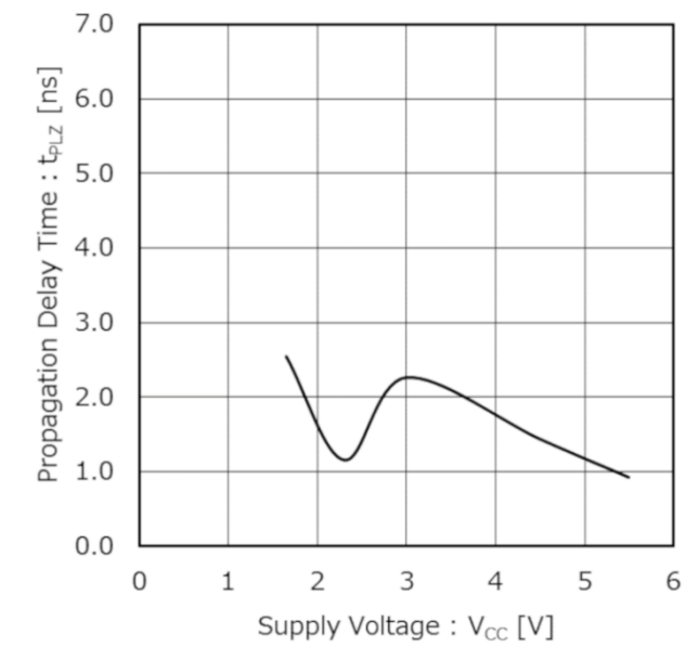
Figure 1. Propagation Delay Time: t_{PLZ} vs Supply Voltage: V_{CC} ( T_a = 25\text{ }^{\circ}\text{C} )
