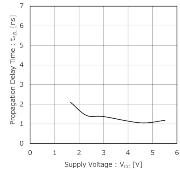
Figure 3. Propagation Delay Time: t_{PZL} vs Supply Voltage: V_{CC} ( T_a = 25\text{ }^{\circ}\text{C} )
