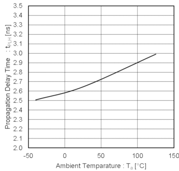
Figure 2. Propagation Delay Time: t_{PLH} vs Ambient Temperature: T_a ( V_{CC} = 3.3\text{ V} ) SS
