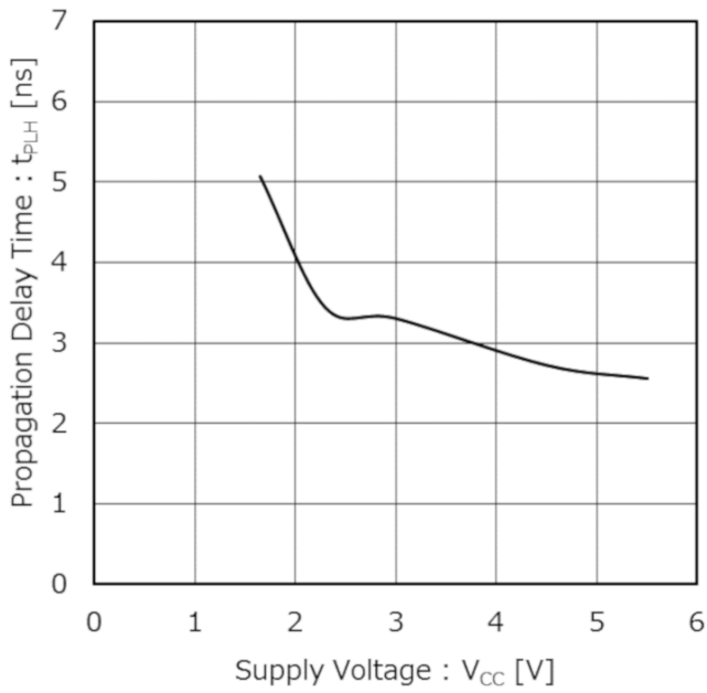
Figure 1. Propagation Delay Time: t PLH vs Supply Voltage: V CC (T a = 25 °C)
