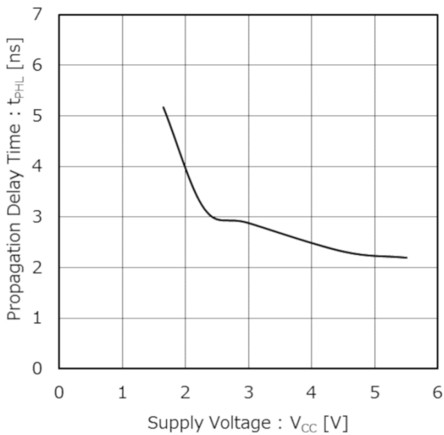
Figure 3. Propagation Delay Time: t PHL vs Supply Voltage: V CC (T a = 25 °C)
