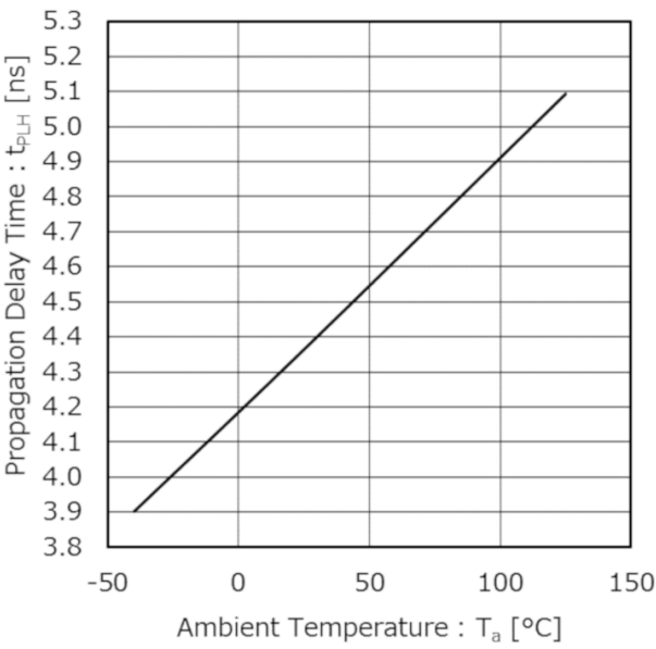
Figure 9. Propagation Delay Time: t_{PLH} vs Ambient Temperature: T_a ( V_{CC} = 3.3\text{ V} )
