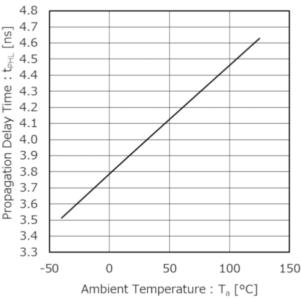
Figure 11. Propagation Delay Time: t_{PHL} vs Ambient Temperature: T_a ( V_{CC} = 3.3\text{ V} )
