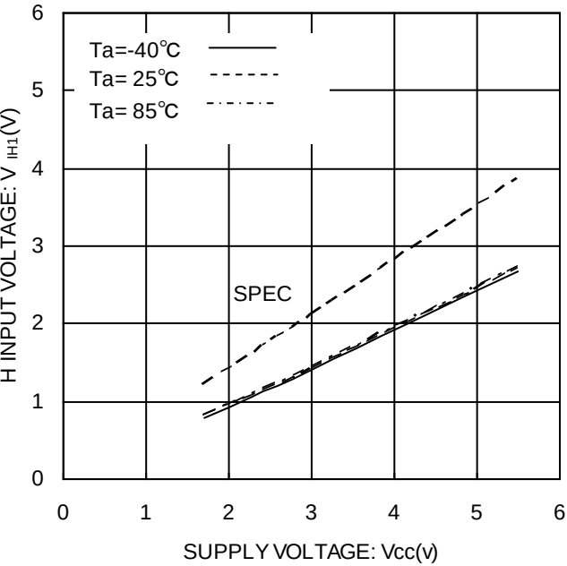
Figure 4. “H”入力電圧 1,2 V_{IH1,2} (A1,A2,SCL,SDA,WP)
