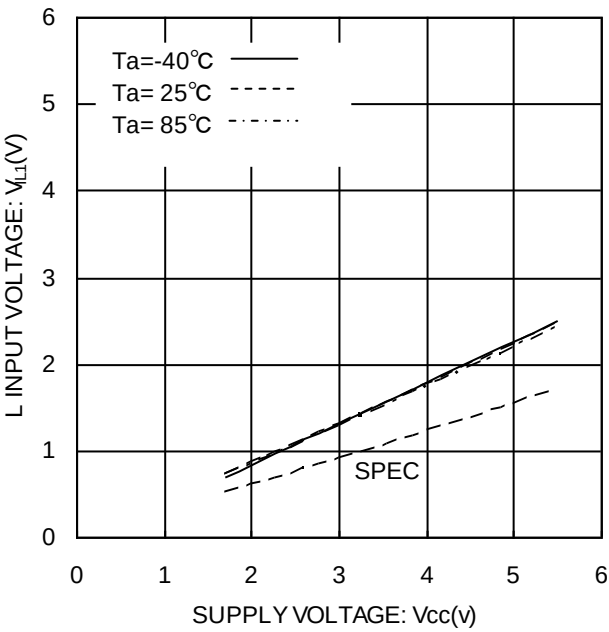
Figure 5. “L”入力電圧 1,2 V_{IL1,2} (A1,A2,SCL,SDA,WP)
