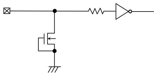
Figure 55. 入力端子回路図 (A1, A2, WP)
