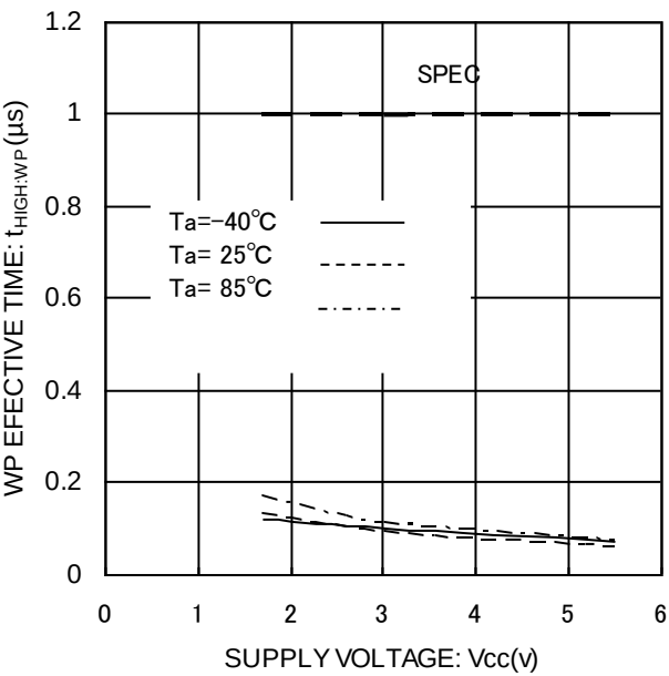
Figure 33. WP 有効時間 t_{HIGH:WP}
