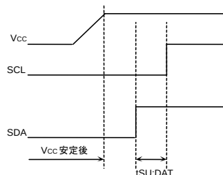
Figure 53. SCL='L' SDA='L'の時
