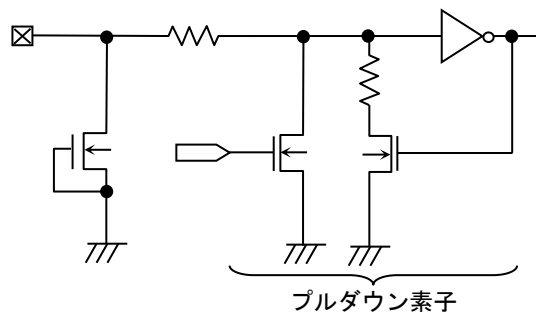
Figure 58. 入力端子回路図 (A2, WP)
