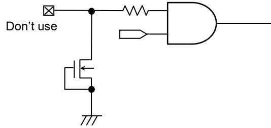
Figure 57. 入力端子回路図 (A0, A1)
