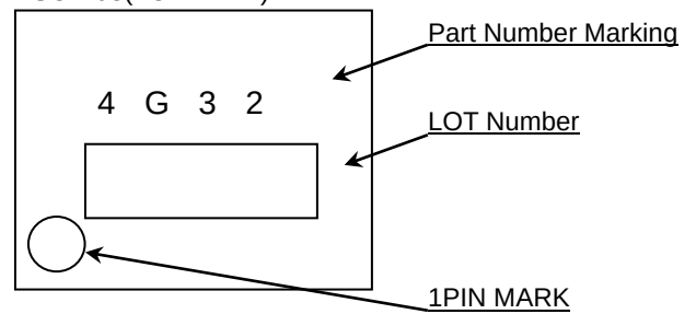
SOP-J8(TOP VIEW)
