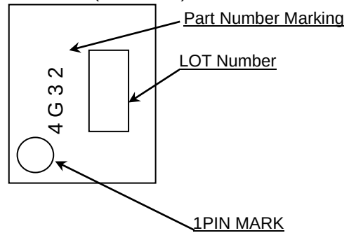
TSSOP-B8(TOP VIEW)
