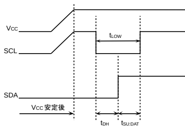
Figure 52. SCL='H' SDA='L'の時
