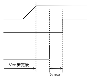
Figure 53. SCL='L' SDA='L'の時
