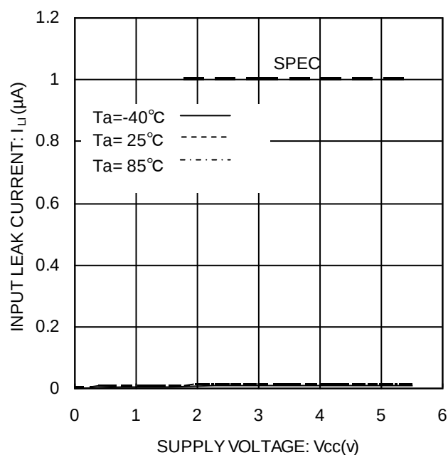
Figure 8. 入力リーク電流 I_{II} (A0,A1,A2,SCL,WP)
