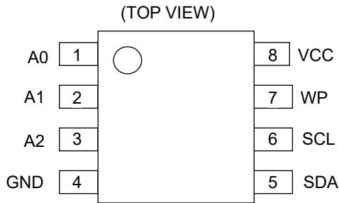
Figure 3-(a). 端子配置図 (SOP8*1、SOP-J8、TSSOP-B8、MSOP8) *1 Not Recommended for New Designs.
