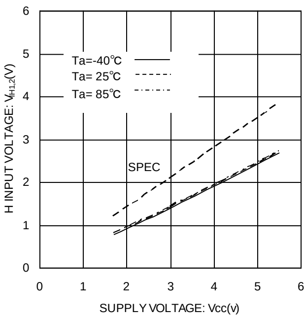
Figure 4. “H”入力電圧 V_{IH1,2} (A0, A1, A2, SCL, SDA, WP)
