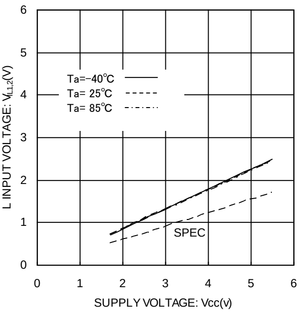
Figure 5. “L”入力電圧 V_{IL1,2} (A0, A1, A2, SCL, SDA, WP)
