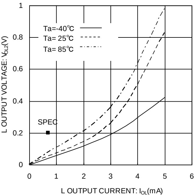
Figure 7. “L”出力電圧 V_{OL2} ( V_{CC} = 1.6\text{V} )
