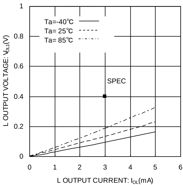
Figure 6. “L”出力電圧 V_{OL1} ( V_{CC} = 2.5\text{V} )
