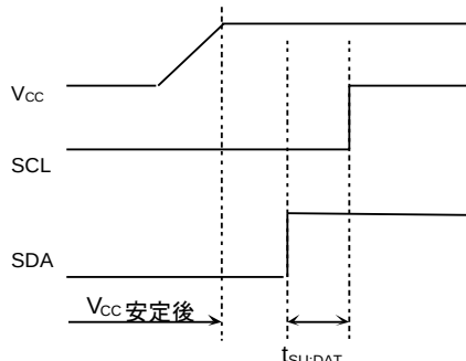
Figure 54. SCL='L' SDA='L'の時
