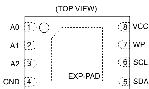
Figure 3-(b). 端子配置図 (VSON008X2030、VSON08AX2030)
