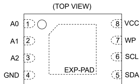
Figure 3-(b). 端子配置図 (VSON008X2030*1、VSON08AX2030) *1 Last Time Buy.
