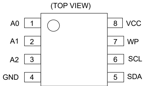
Figure 3-(a). 端子配置図 (SOP8*1、SOP-J8、TSSOP-B8、MSOP8) *1 Last Time Buy.
