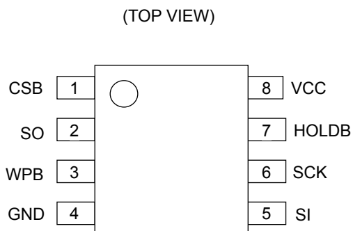
Figure 3. 端子配置図 (SOP-J8、TSSOP-B8)
