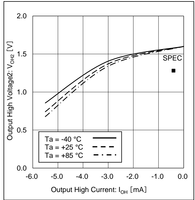
Figure 12. 'HIGH'出力電圧 2 vs 'HIGH'出力電流 ( V_{CC} = 1.6 \text{ V} )
