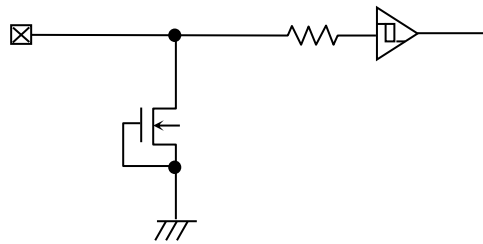
Figure 59. 入力端子回路図 (CSB, SCK, SI, HOLDB, WPB)
