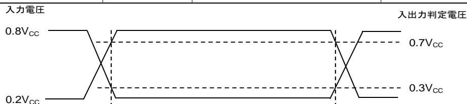
Figure 5. 入出力判定電圧
