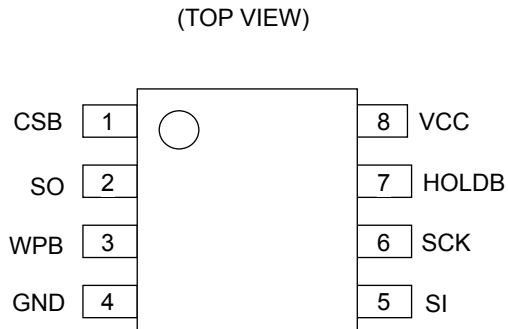
Figure 3. 端子配置図 (SOP-J8、TSSOP-B8、MSOP8)
