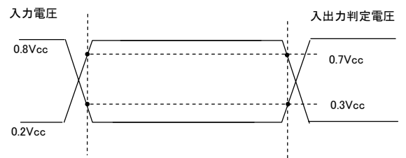
Figure 1. 入出力判定電圧
