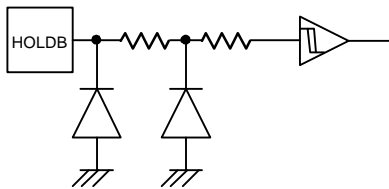
Figure 58. HOLDB 入力等価回路
