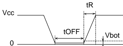
Figure 61. 立ち上がり波形
