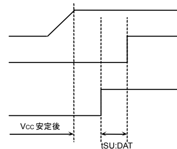
Figure 54. SCL='H' SDA='L'の時
