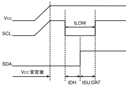
Figure 53. SCL='H' SDA='L'の時
