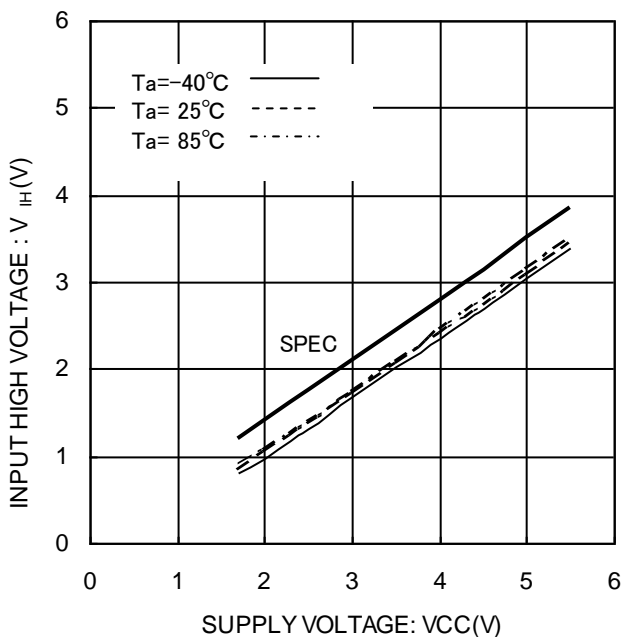
Figure 4. “H”入力電圧 V_{IH} (CS,SK,DI)
