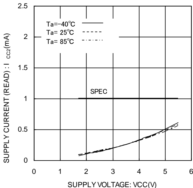
Figure 17. READ 動作時消費電流 I cc2 (READ, f sk =3MHz)
