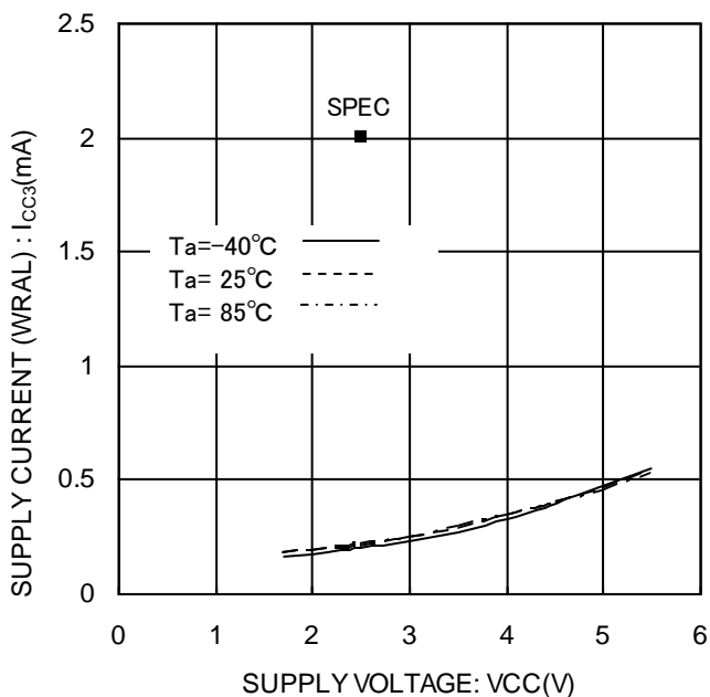
Figure 18. WRAL 動作時消費電流 I cc3 (WRAL, f sk =1MHz)
