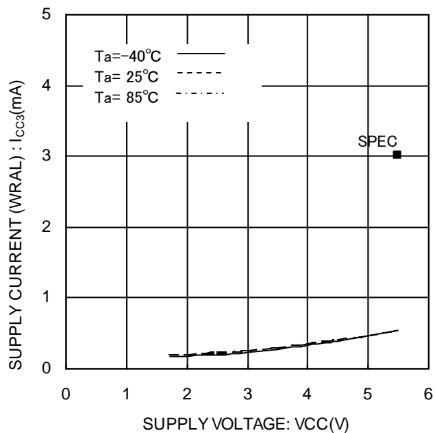
Figure 19. WRAL 動作時消費電流 I cc3 (WRAL, f sk =3MHz)
