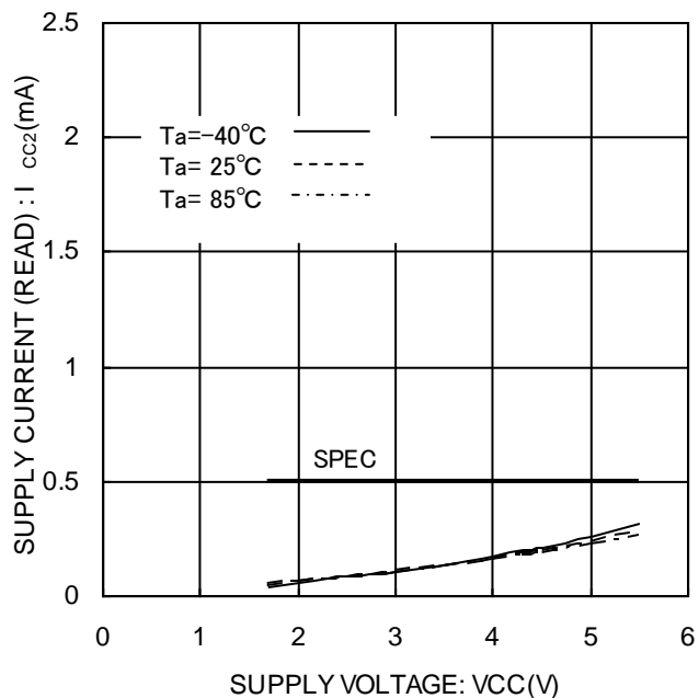
Figure 16. READ 動作時消費電流 I cc2 (READ, f sk =1MHz)
