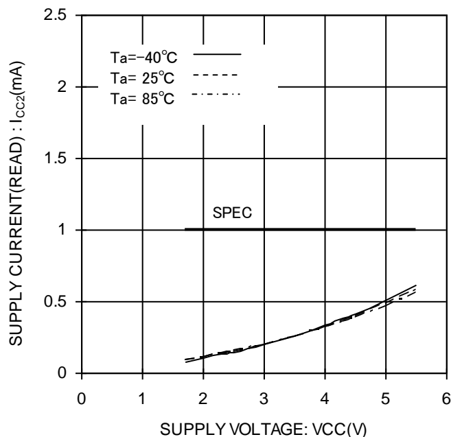
Figure 17. READ 動作時消費電流 Icc2(READ,fsk=3MHz)
