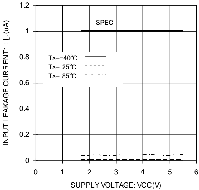
Figure 12. 入力リーク電流 1 I_{L1}(DI)
