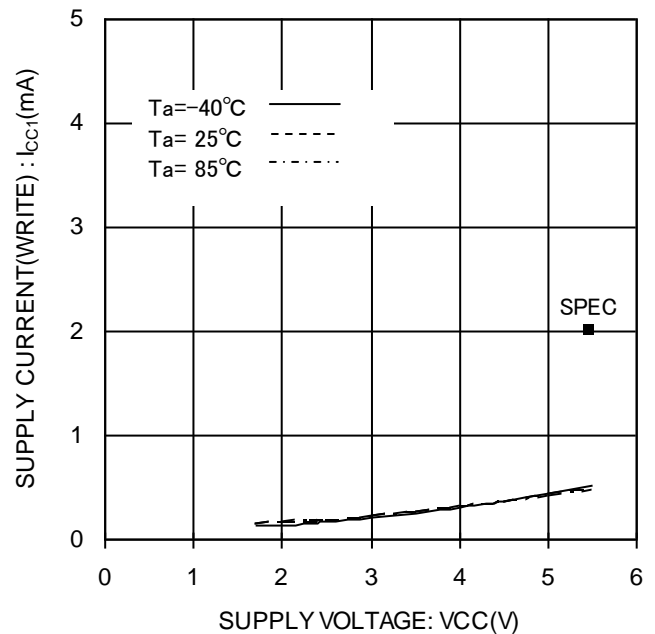
Figure 15. WRITE 動作時消費電流 I_{CC1}(WRITE, f_{sk}=3MHz)
